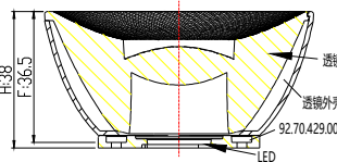
OPTICAL ASSEMBLY DIAGRAM
