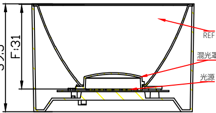
OPTICAL ASSEMBLY DIAGRAM
