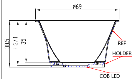
OPTICAL ASSEMBLY DIAGRAM
