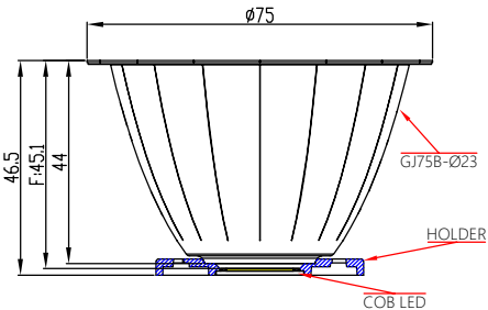
OPTICAL ASSEMBLY DIAGRAM
