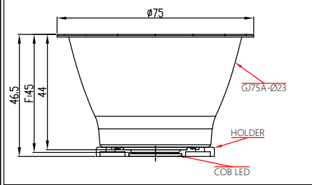
OPTICAL ASSEMBLY DIAGRAM
