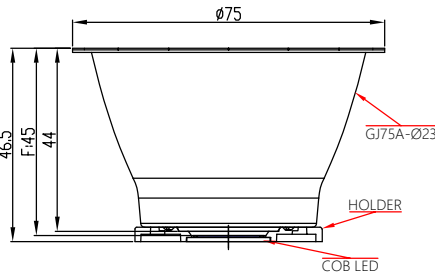
OPTICAL ASSEMBLY DIAGRAM
