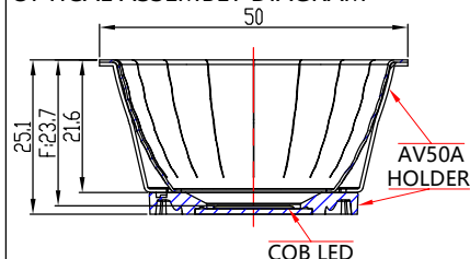
OPTICAL ASSEMBLY DIAGRAM
