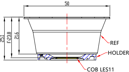
OPTICAL ASSEMBLY DIAGRAM
