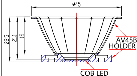
OPTICAL ASSEMBLY DIAGRAM
