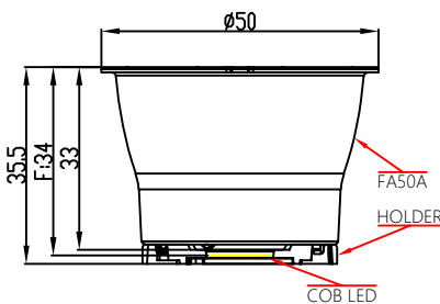
OPTICAL ASSEMBLY DIAGRAM
