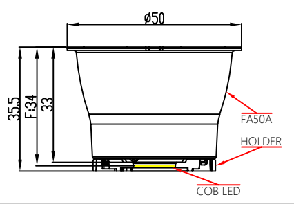
OPTICAL ASSEMBLY DIAGRAM
